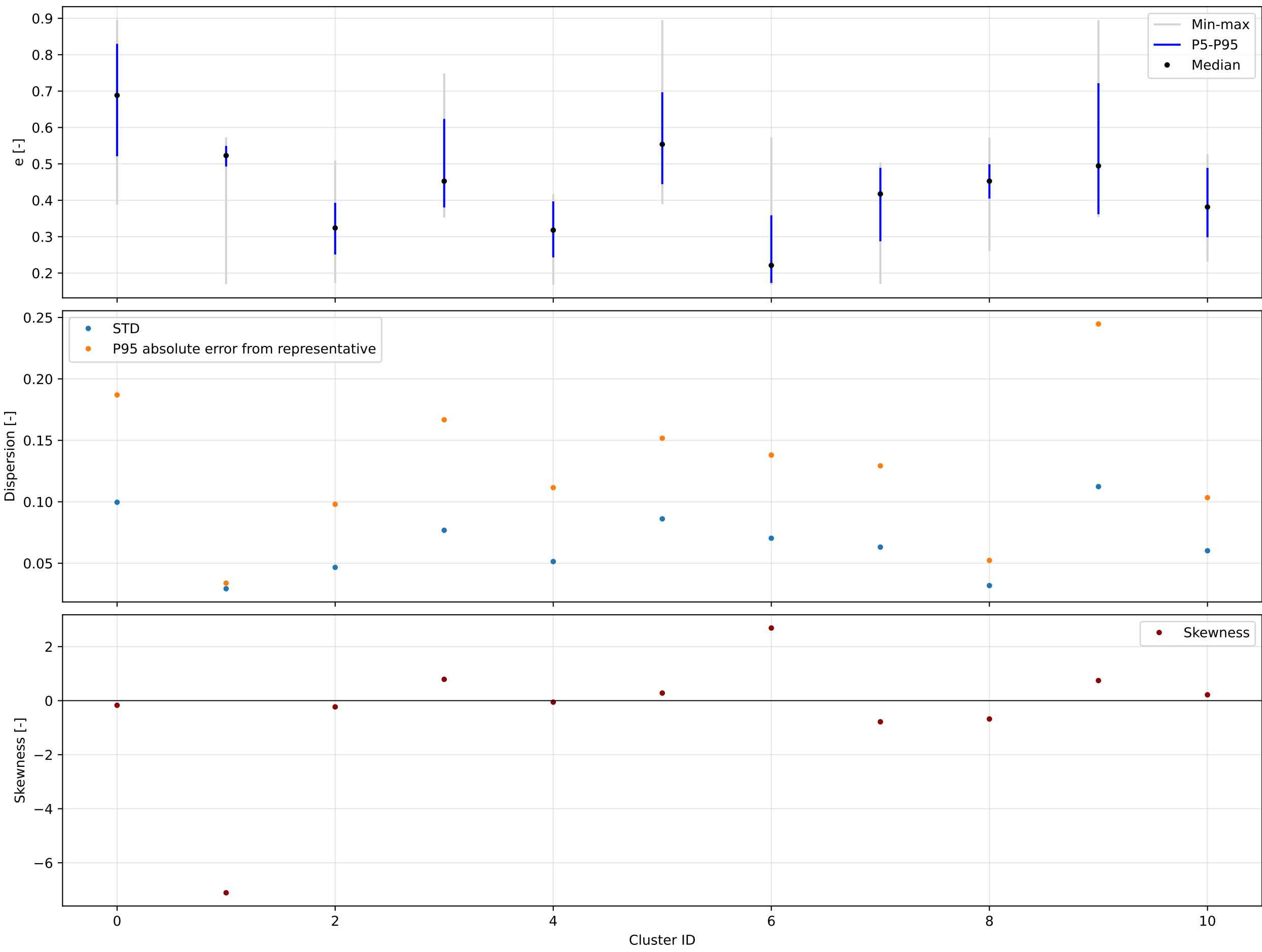
K=11 | backward | e | valid=194124/194124
