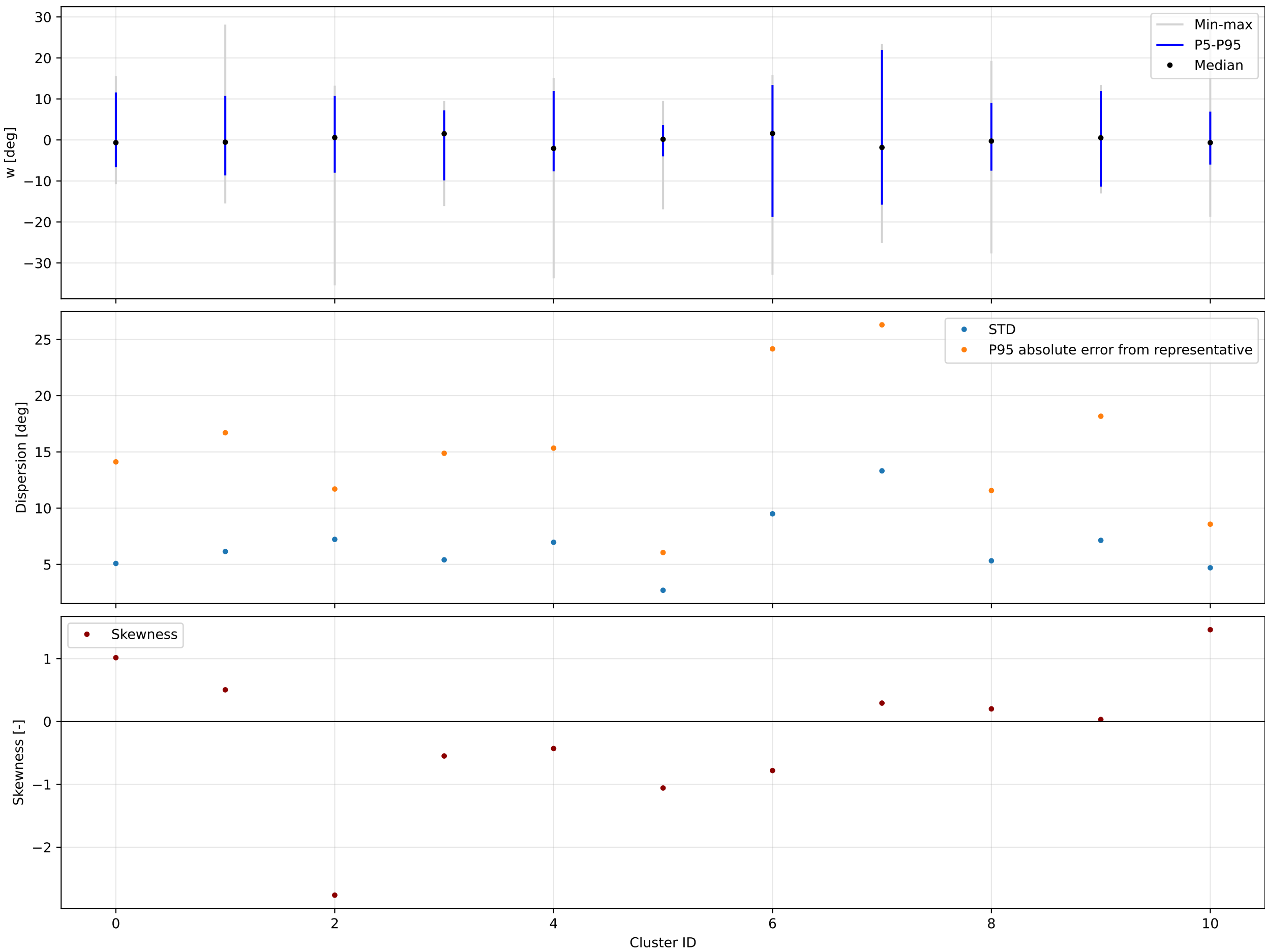
K=11 | backward | w | valid=194124/194124 | offsets from each cluster circular mean
