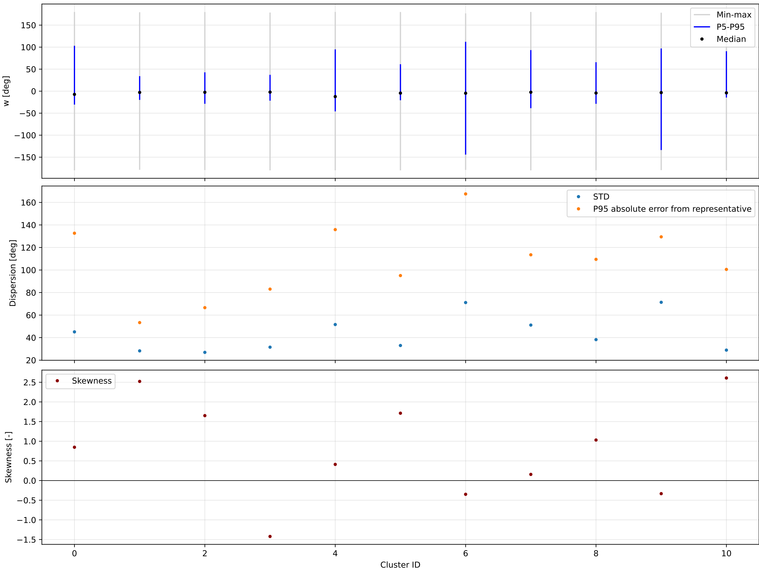
K=11 | forward | w | valid=194058/194124 | offsets from each cluster circular mean
